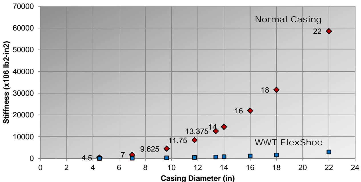
Casing Size vs. Stiffness
